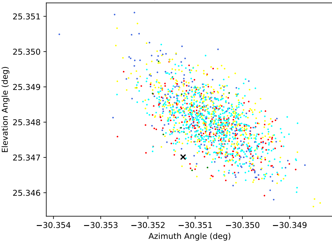
Timestep 16.9338 Hours (Post)
